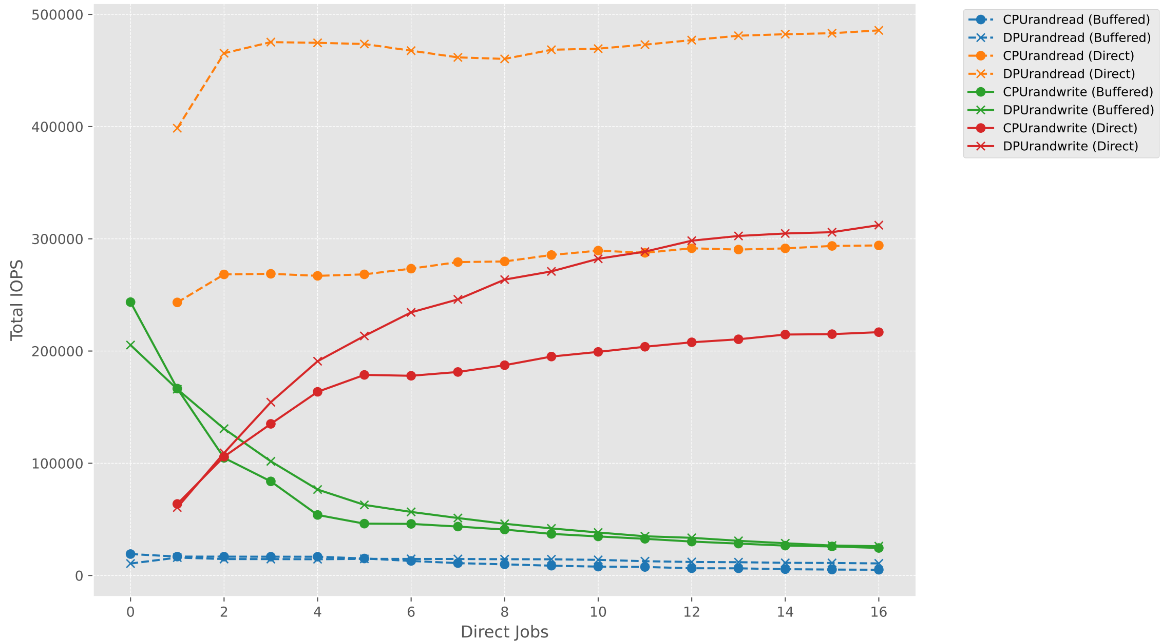
IOPS vs Direct Jobs (buffered1_directN) - RAND (CPU vs DPU)
